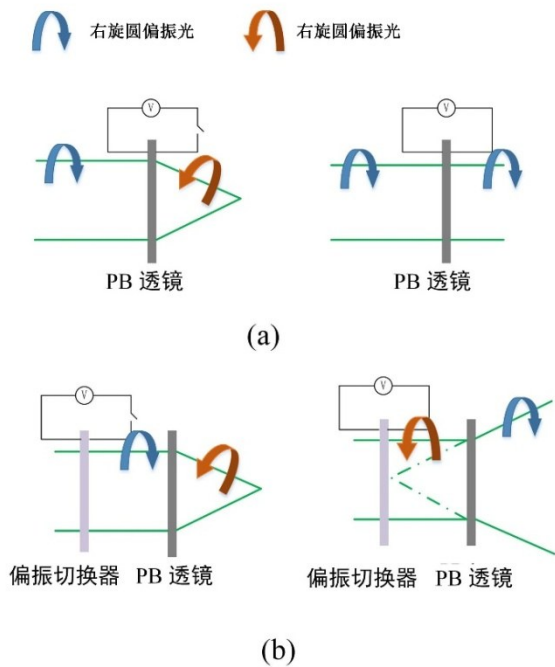
图11 PB透镜的两种驱动方式:(a)主动驱动方式,(b)被动驱动方式 Fig. 11 Two driving methods for a PB lens: (a) active driving method and (b) passive driving method
