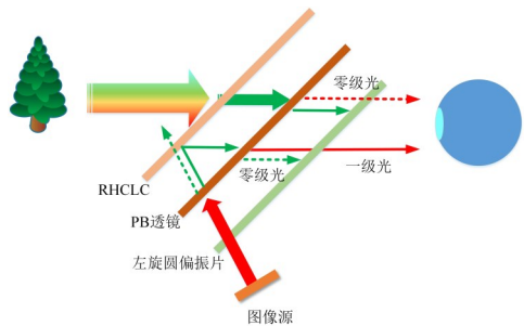
图12基于PB透镜的抬头显示系统设计 Fig. 12 System design of the head up display based on a PB lens
